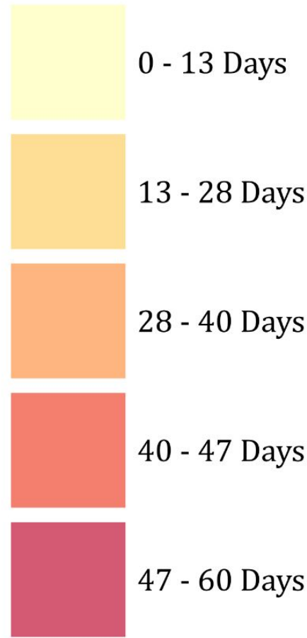
RCP 8.5 Ensemble Mean Projections Data derived from LOCA Downscaled CMIP5 Projections.
